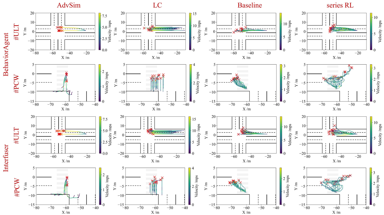
Fig. 10. Scenario repository of the trajectories for the four adversarial policies.
