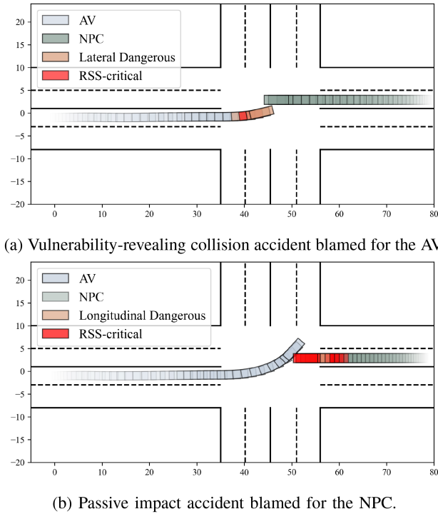
Fig. 3. Collision accidents under the unprotected left turn driving task blamed for the opposite entities. The vehicle state is represented by the rectangles of different colors, the orange is referred to dangerous states and the red is referred to RSS-critical frame.
