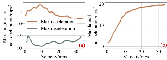
Fig. 6. Calibrations of (a) the max longitudinal acc-deceleration and (b) the max lateral acceleration for Carla Lincoln MKZ-2017.
