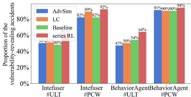
Fig. 9. Proportion of the vulnerability-revealing accidents among all scenarios.
