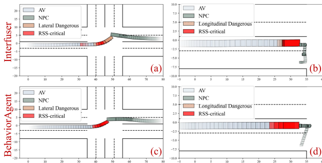
Fig. 11. Vulnerability-revealing accidents for Interfuser under (a) #ULT and (b) #PCW and BehaviorAgent under (c) #ULT and (d) #PCW.
